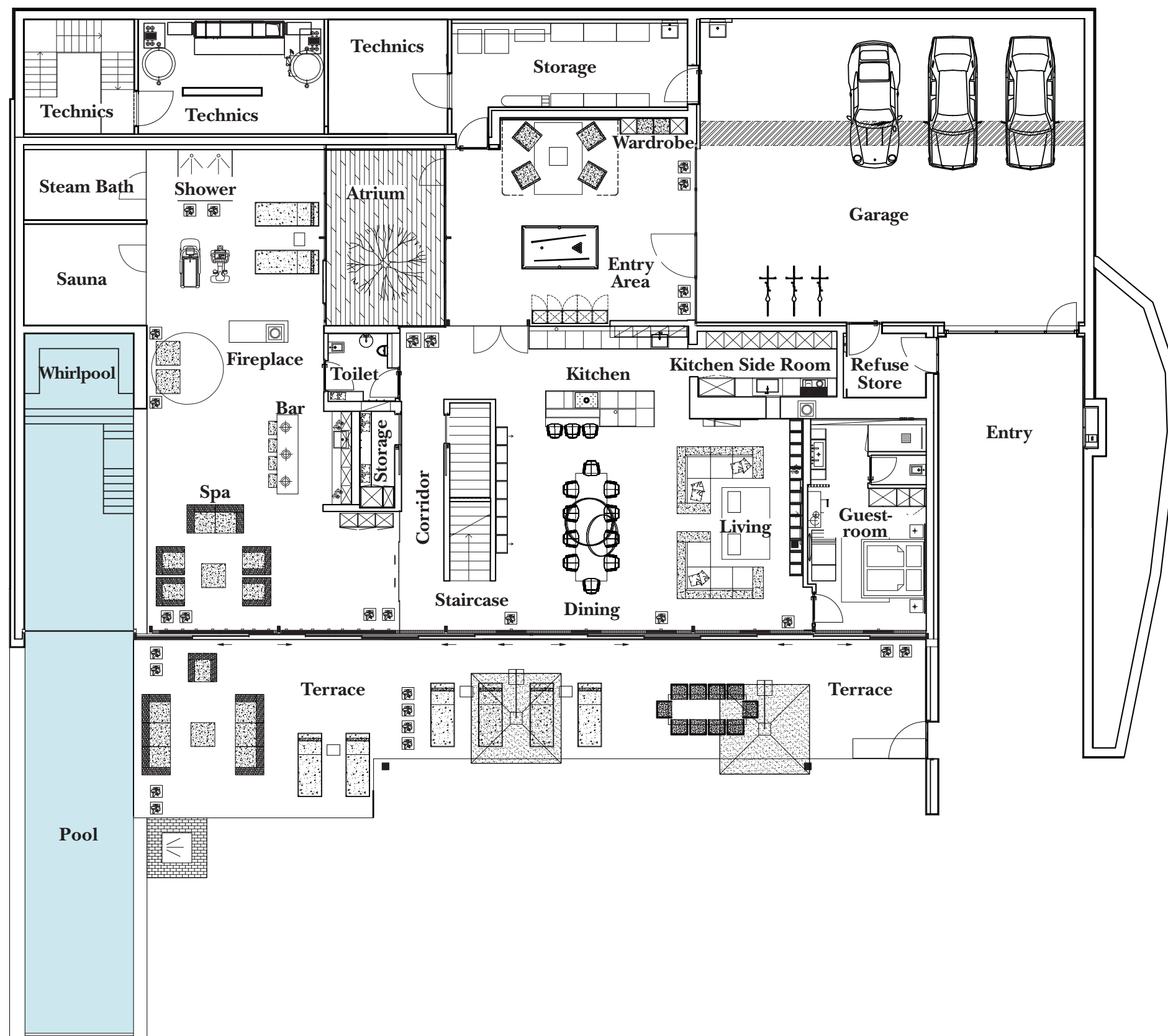
Ground Floor VILLA SPHERE NORD
